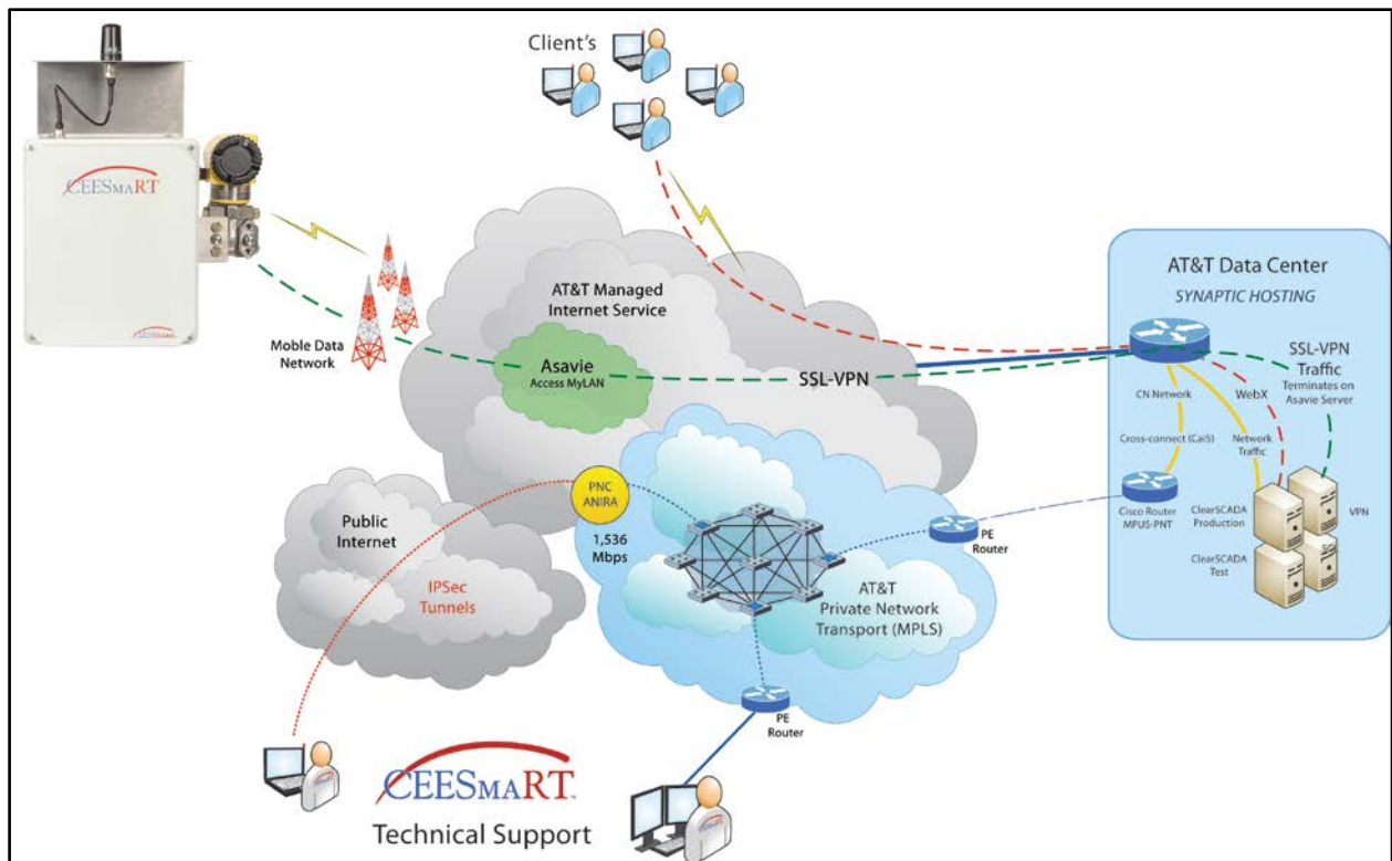
Figure 2 - Overall System Communication Topology
