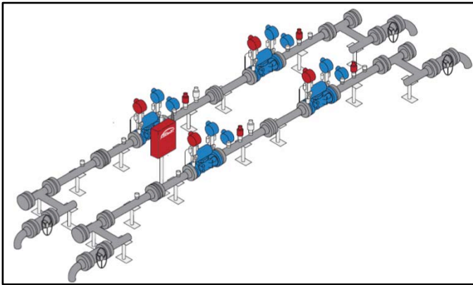
Figure 1 - Dual Meter Runs in Series/Parallel
