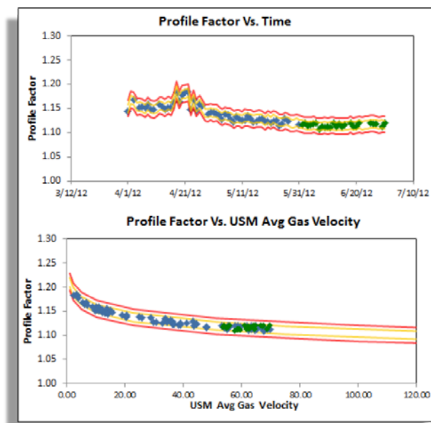
Figure 6 – USM Profile Factor Example
