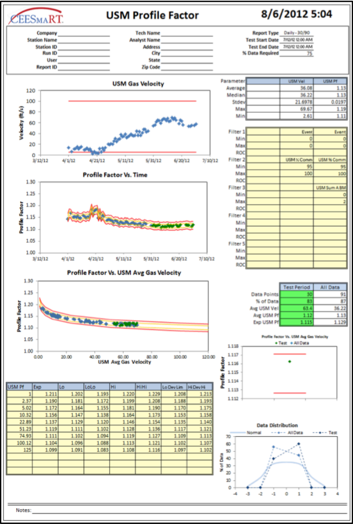
Figure 5 – USM Profile Factor Example
